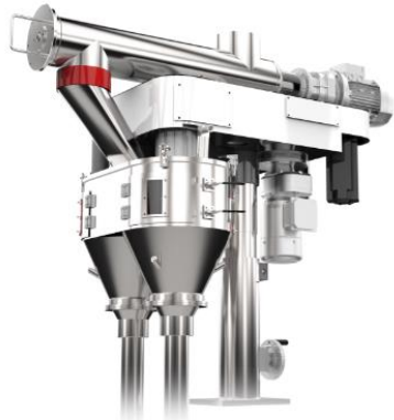
ROVEMA Accu Screw Auger Filler FB280J equipped with TCF & Twin Auger Filler An ideal choice for Oats & Seasoning Packaging - YouTube
